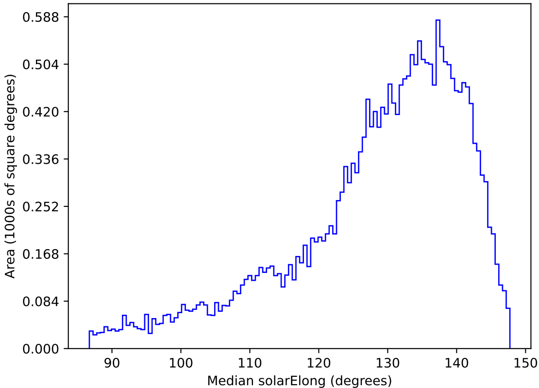
too_5_4v3.4_10yrs All sky y band: Median solarElong
