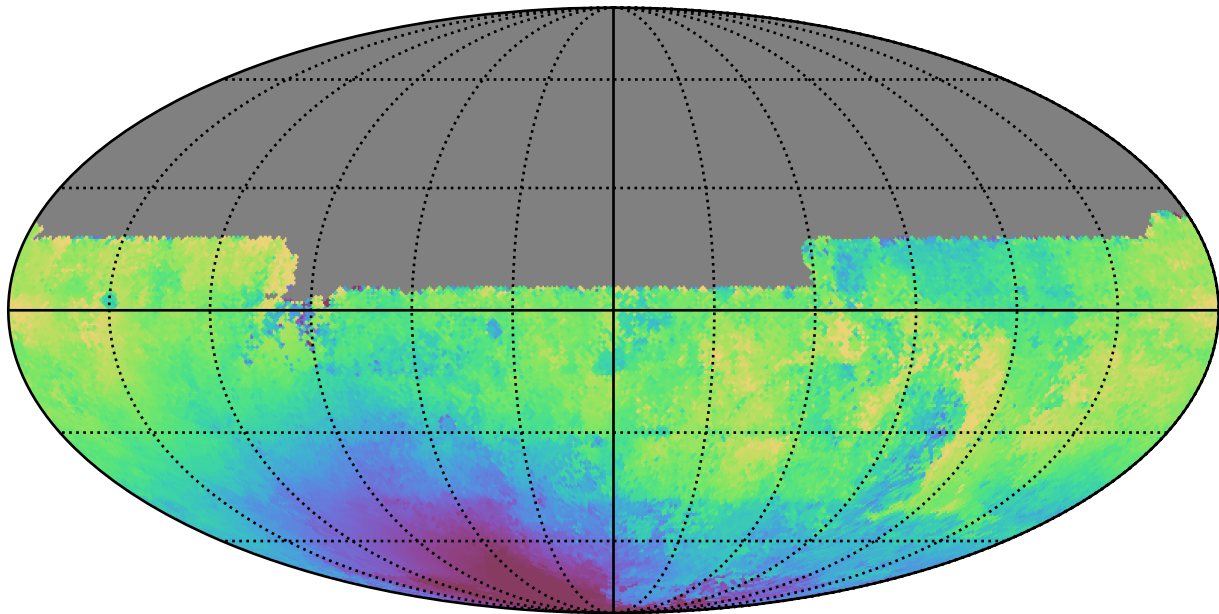
too_5_4v3.4_10yrs All sky u band: Median solarElong
