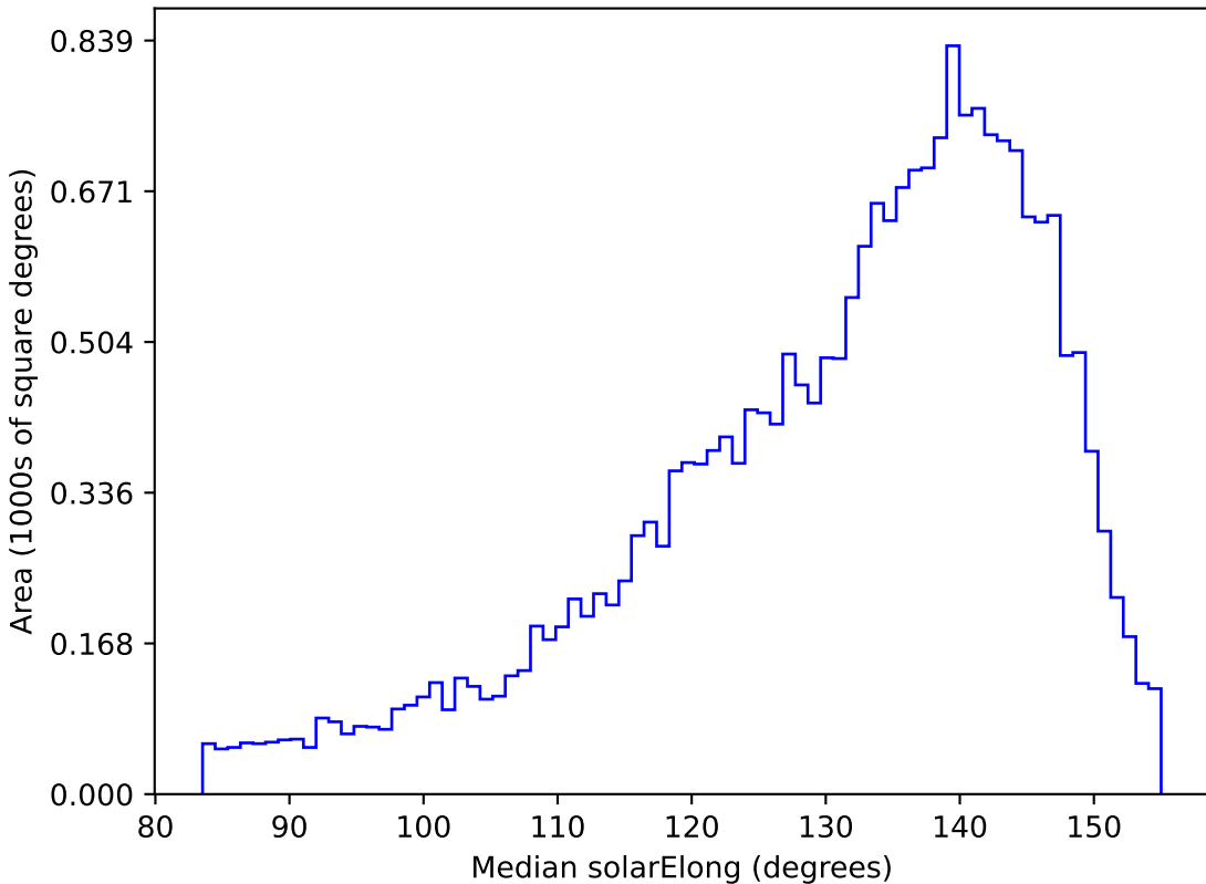
too_5_4v3.4_10yrs All sky u band: Median solarElong
