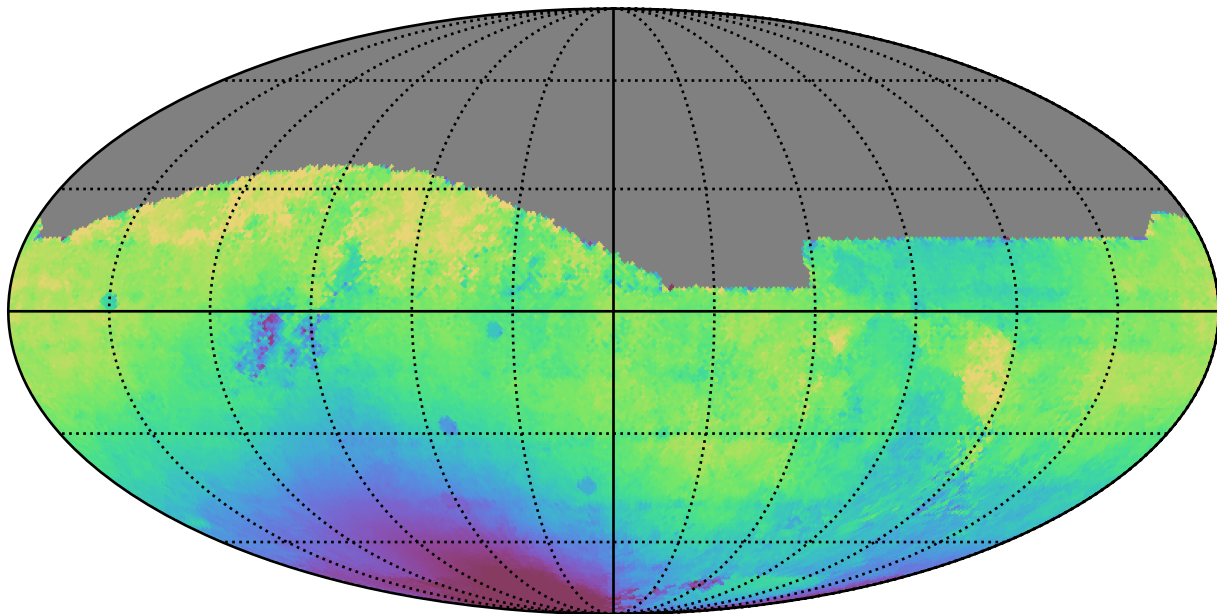
too_5_4v3.4_10yrs All sky r band: Median solarElong
