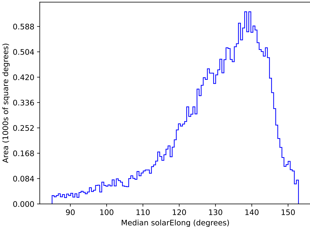
too_5_4v3.4_10yrs All sky r band: Median solarElong
