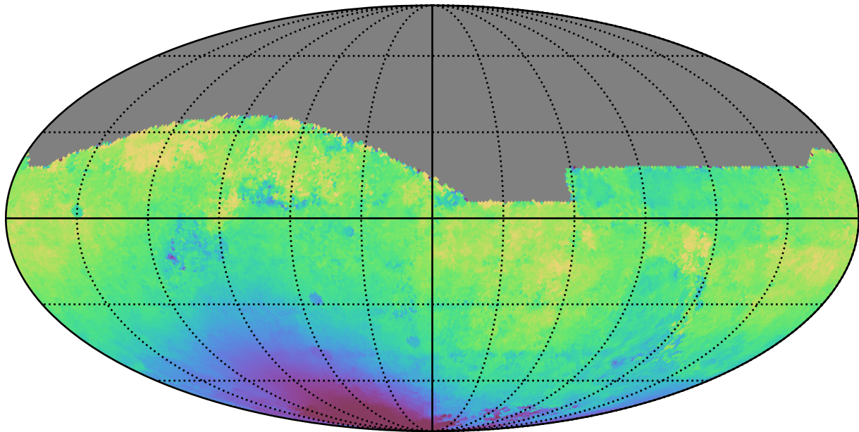
too_5_4v3.4_10yrs All sky i band: Median solarElong
