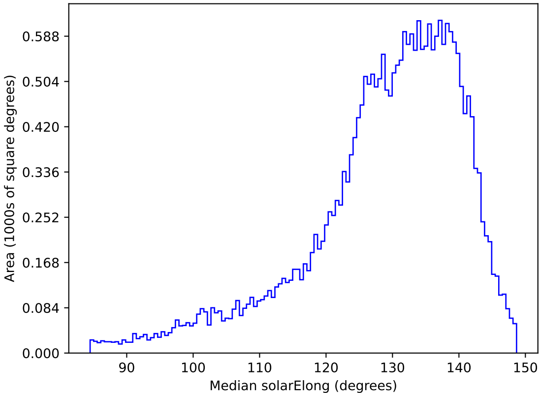
too_5_4v3.4_10yrs All sky i band: Median solarElong
