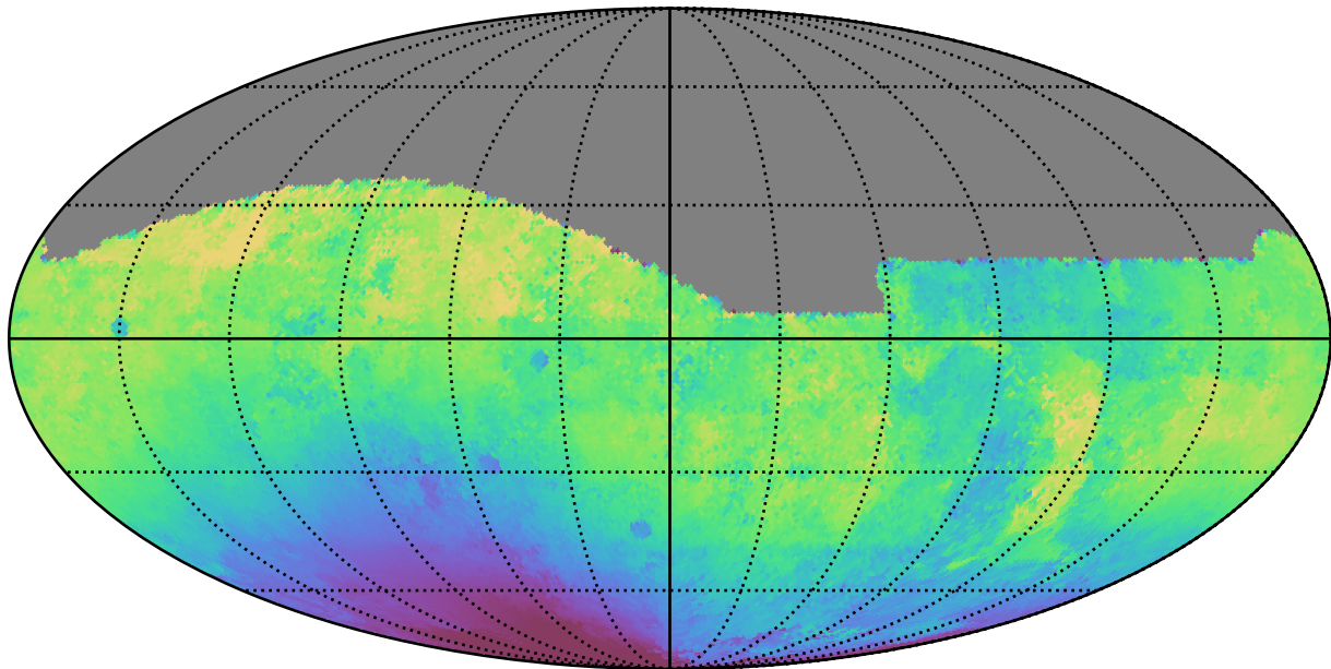
too_5_4v3.4_10yrs All sky g band: Median solarElong
