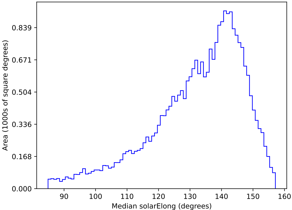
too_5_4v3.4_10yrs All sky g band: Median solarElong
