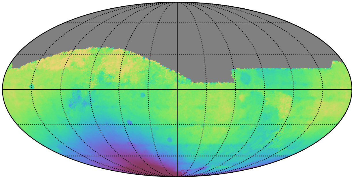
too_5_4v3.4_10yrs All sky all bands: Median solarElong
