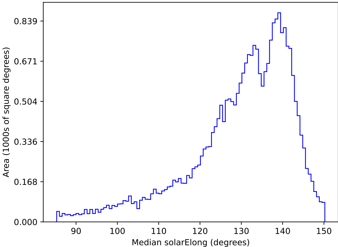
too_5_4v3.4_10yrs All sky all bands: Median solarElong
