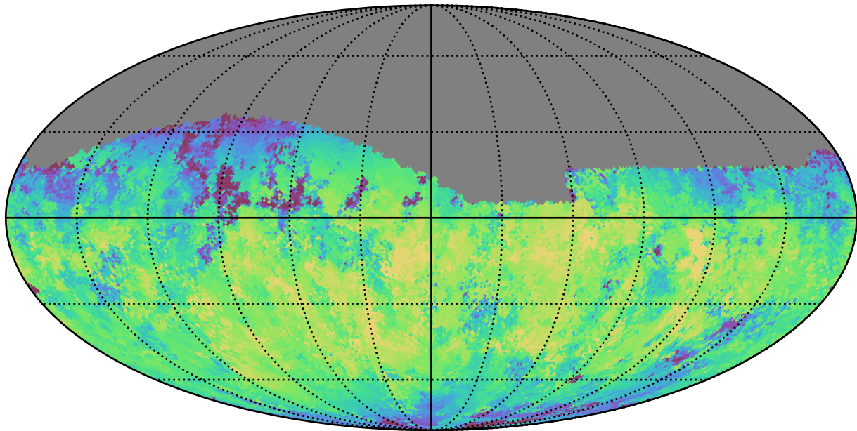
too_5_4v3.4_10yrs Yr 1 z band: Median skyBrightness
