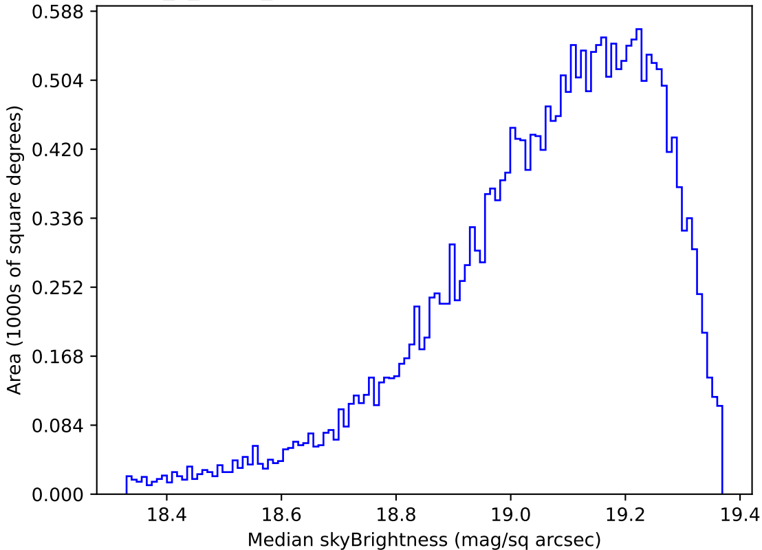
too_5_4v3.4_10yrs Yr 1 z band: Median skyBrightness
