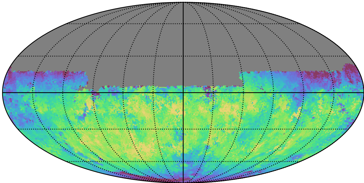
too_5_4v3.4_10yrs Yr 1 y band: Median skyBrightness
