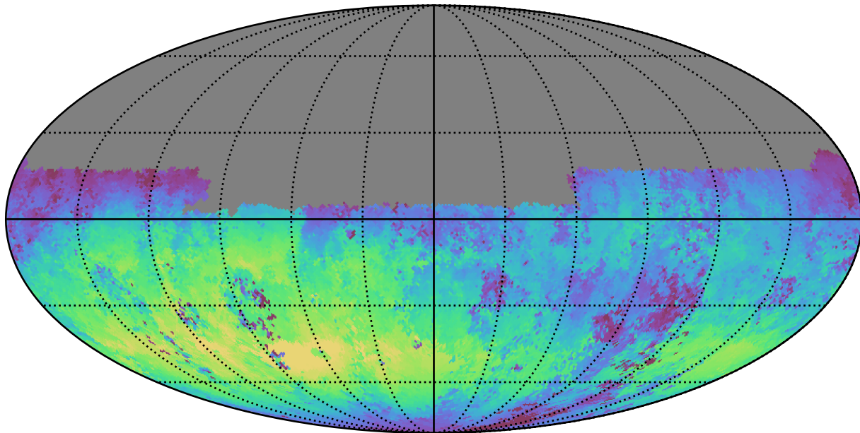
too_5_4v3.4_10yrs Yr 1 u band: Median skyBrightness
