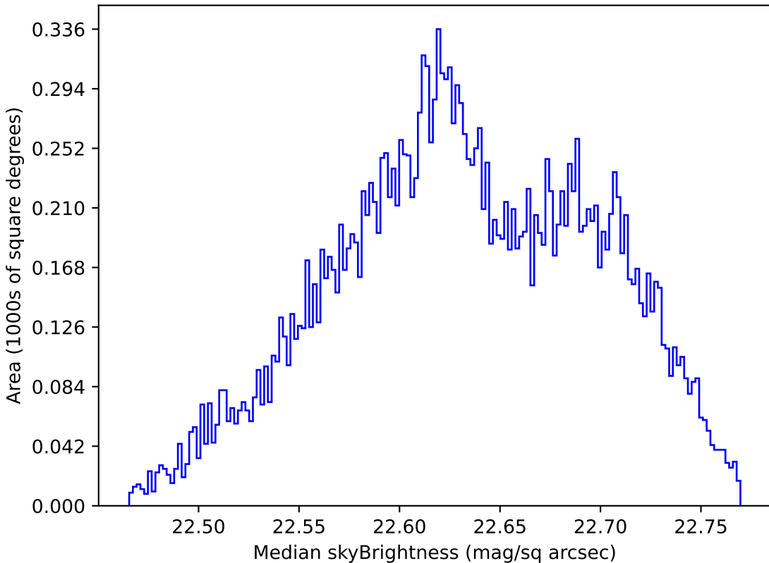
too_5_4v3.4_10yrs Yr 1 u band: Median skyBrightness
