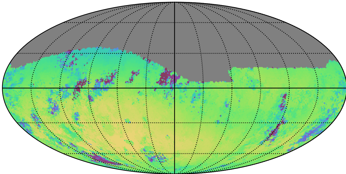
too_5_4v3.4_10yrs Yr 1 r band: Median skyBrightness
