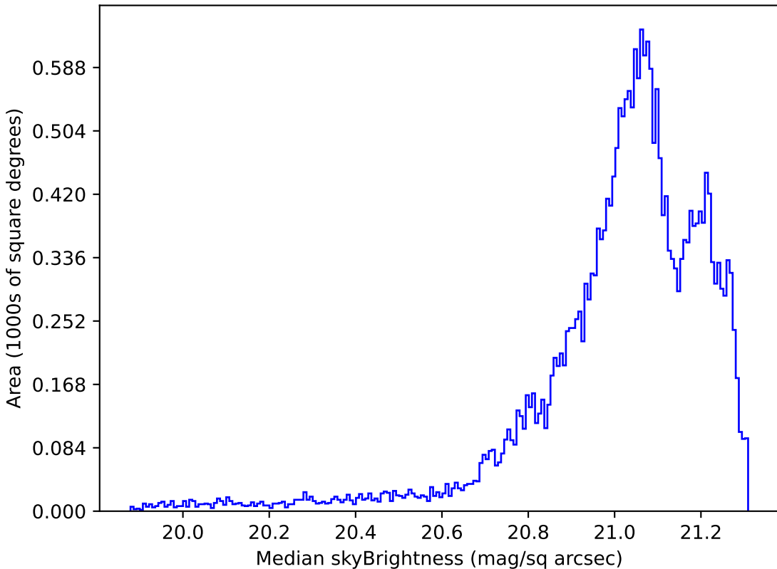
too_5_4v3.4_10yrs Yr 1 r band: Median skyBrightness
