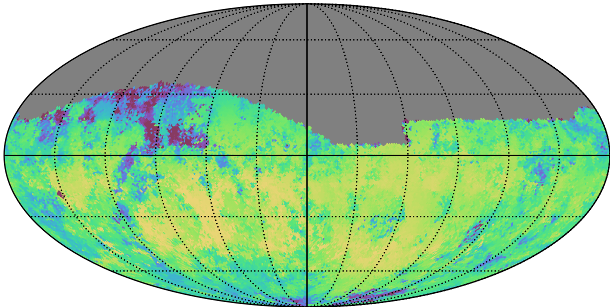
too_5_4v3.4_10yrs Yr 1 i band: Median skyBrightness
