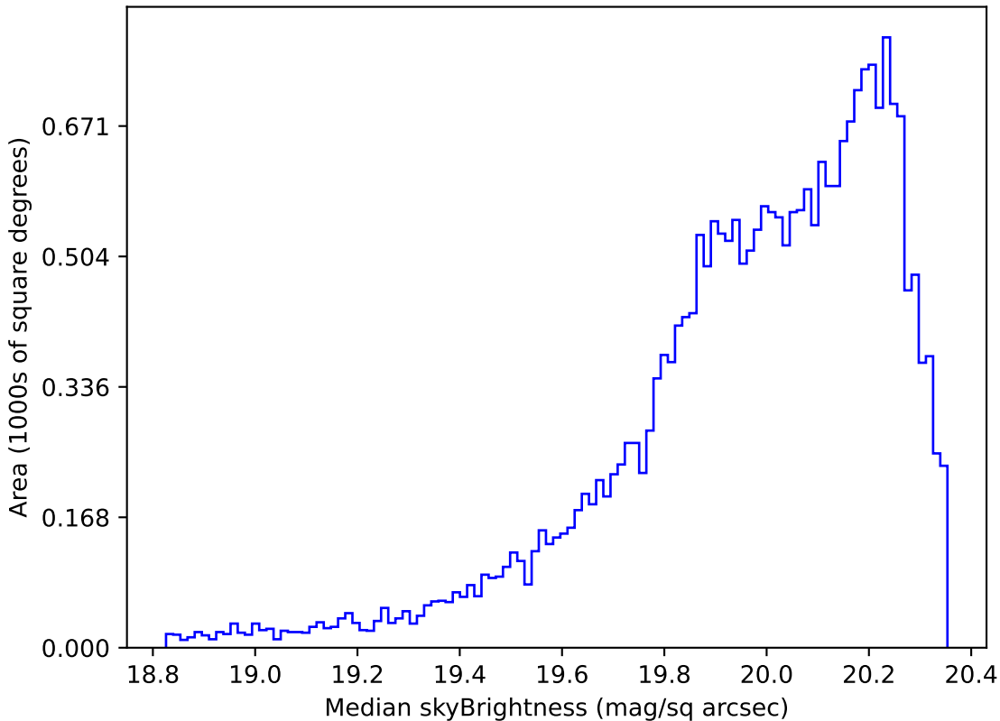
too_5_4v3.4_10yrs Yr 1 i band: Median skyBrightness
