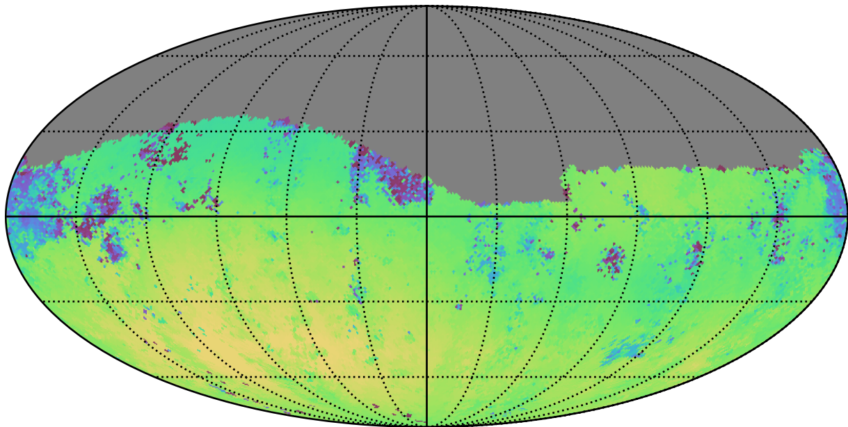
too_5_4v3.4_10yrs Yr 1 g band: Median skyBrightness
