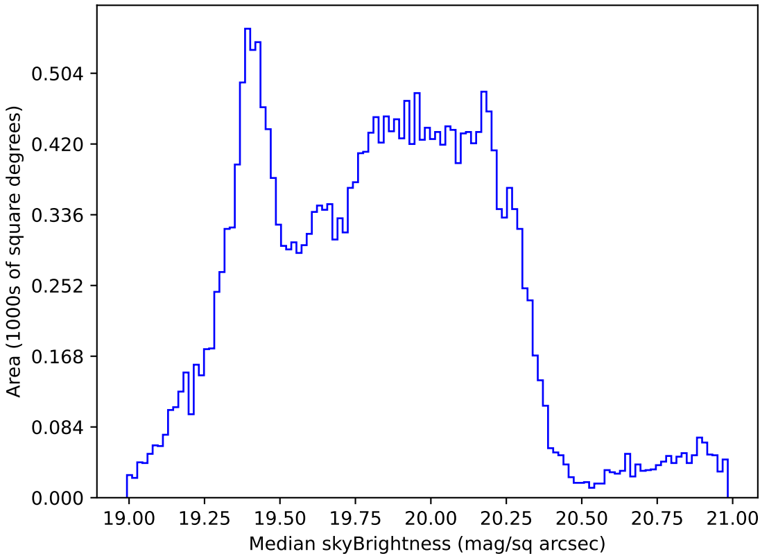
too_5_4v3.4_10yrs Yr 1 all bands: Median skyBrightness
