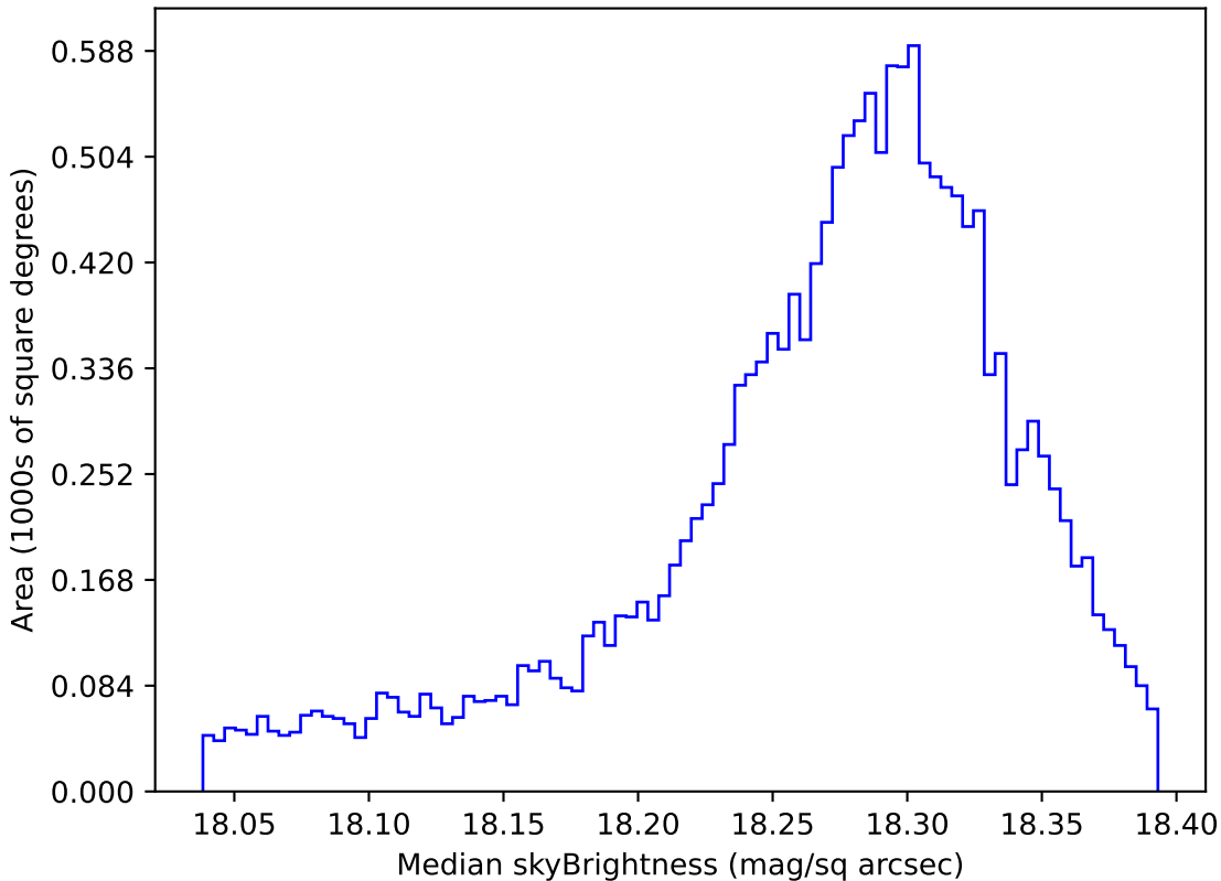
too_5_4v3.4_10yrs WFD y band: Median skyBrightness
