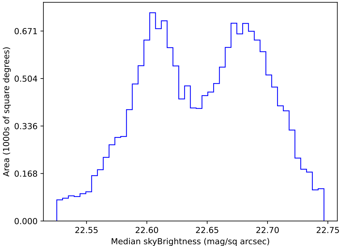
too_5_4v3.4_10yrs WFD u band: Median skyBrightness
