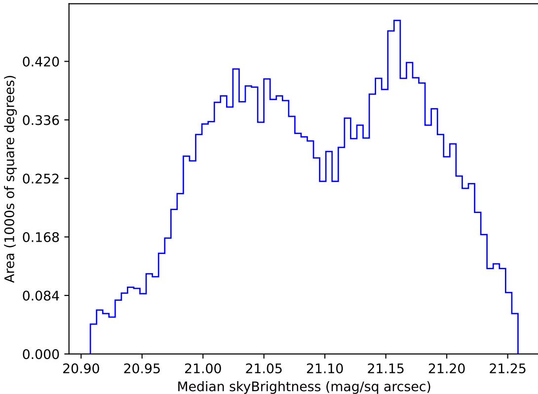
too_5_4v3.4_10yrs WFD r band: Median skyBrightness
