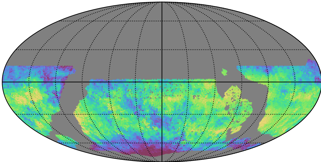
too_5_4v3.4_10yrs WFD i band: Median skyBrightness
