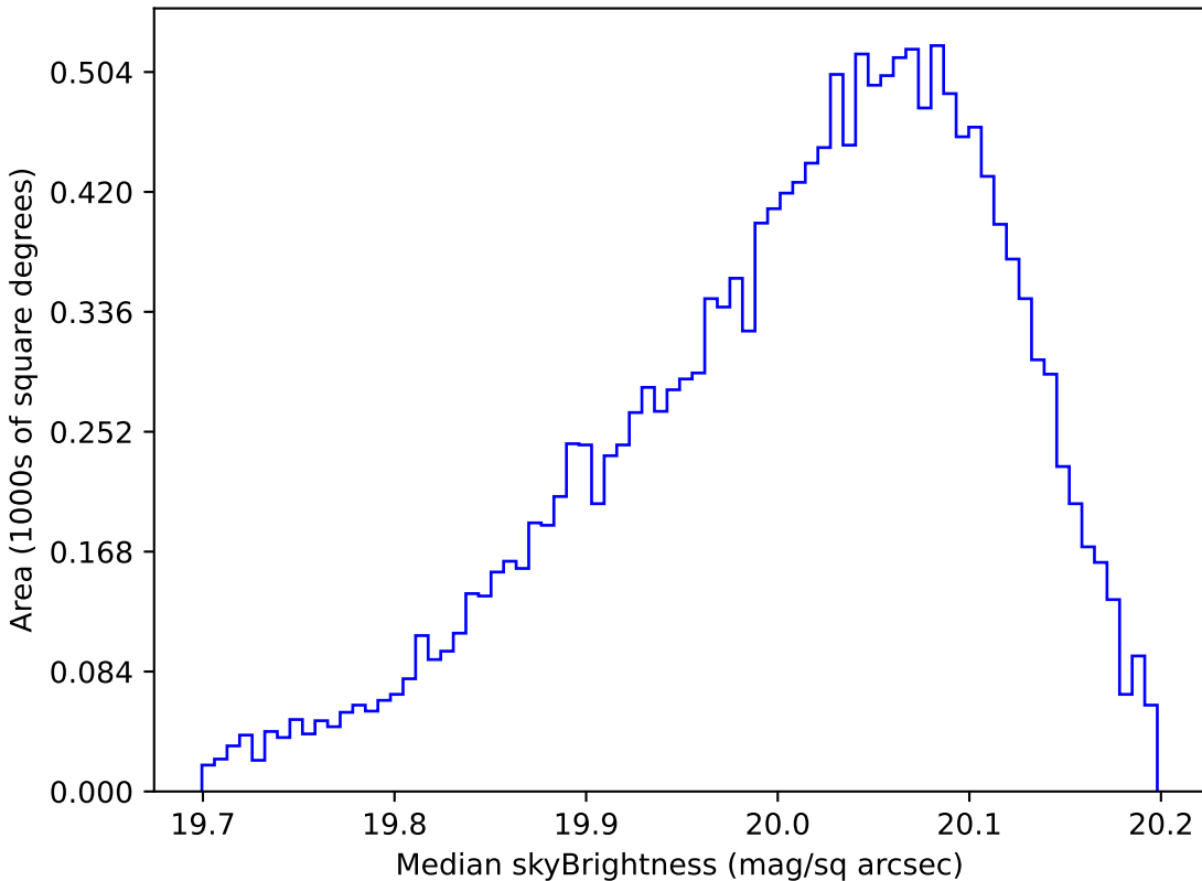
too_5_4v3.4_10yrs WFD i band: Median skyBrightness
