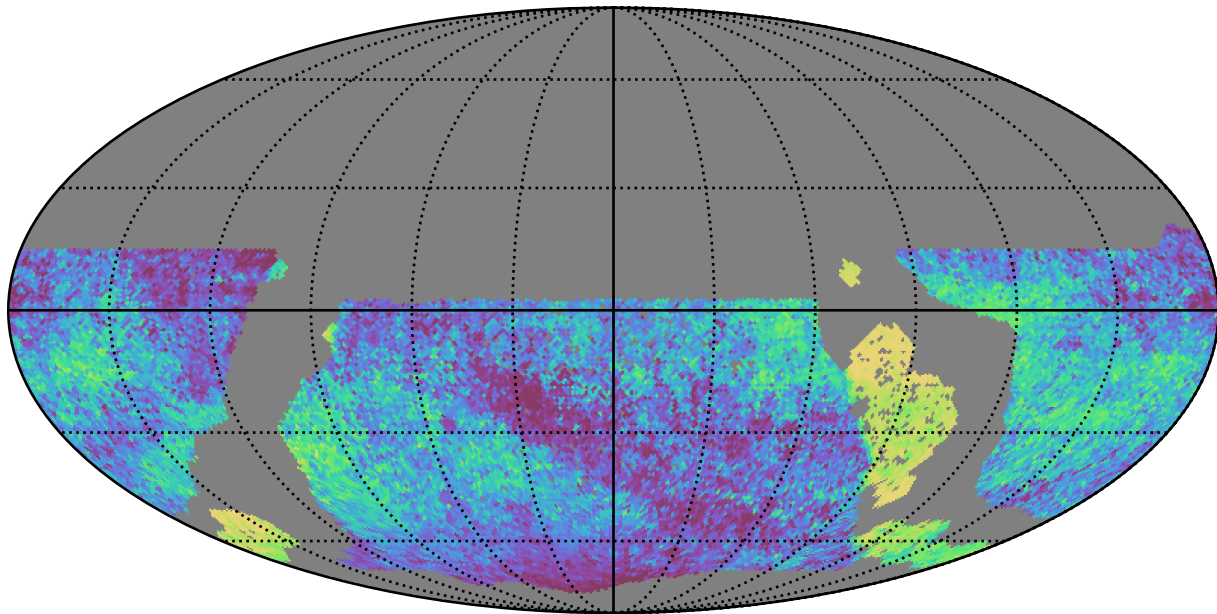
too_5_4v3.4_10yrs WFD all bands: Median skyBrightness
