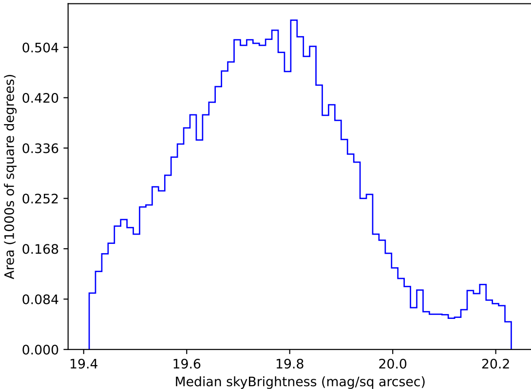
too_5_4v3.4_10yrs WFD all bands: Median skyBrightness
