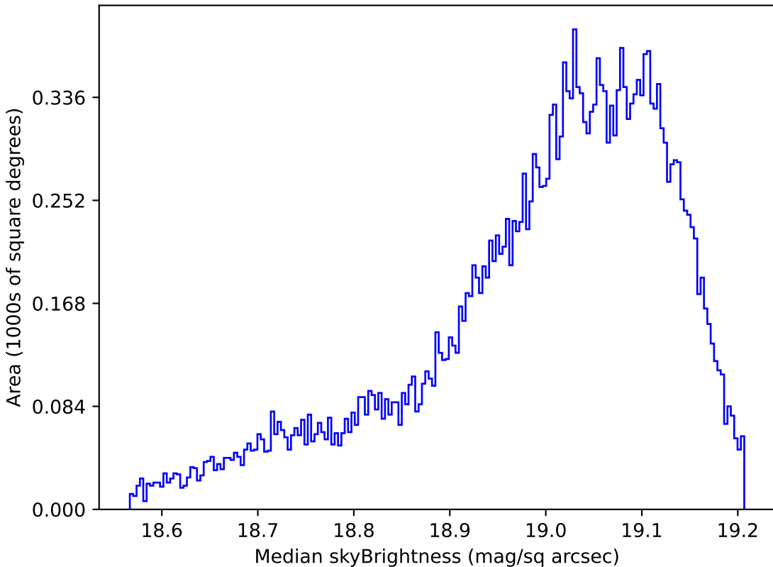
too_5_4v3.4_10yrs All sky z band: Median skyBrightness
