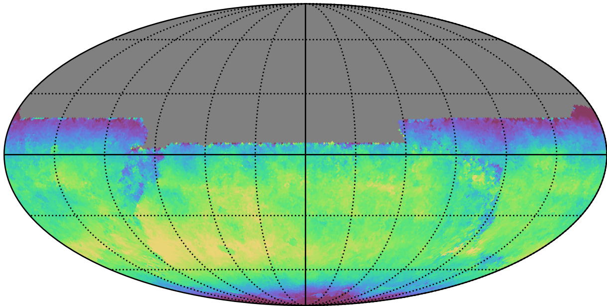
too_5_4v3.4_10yrs All sky y band: Median skyBrightness
