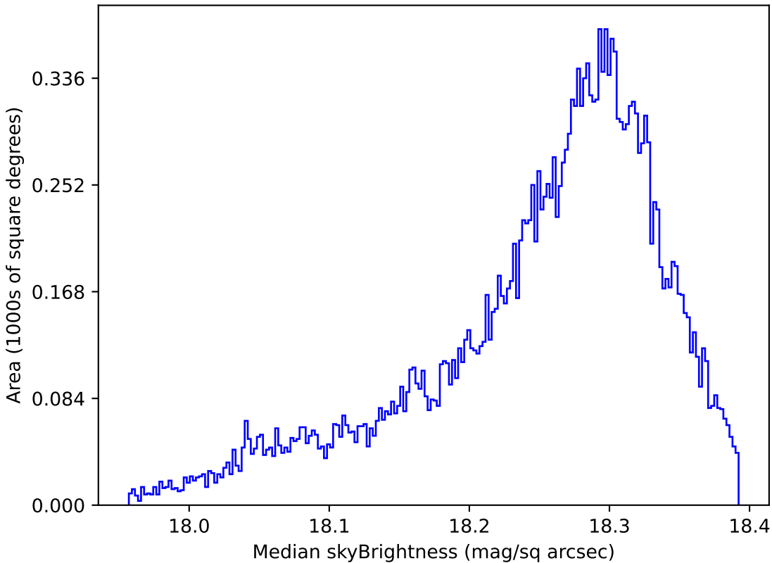
too_5_4v3.4_10yrs All sky y band: Median skyBrightness
