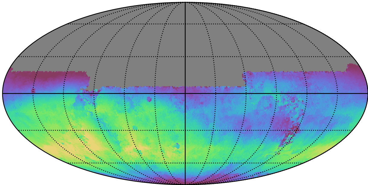
too_5_4v3.4_10yrs All sky u band: Median skyBrightness
