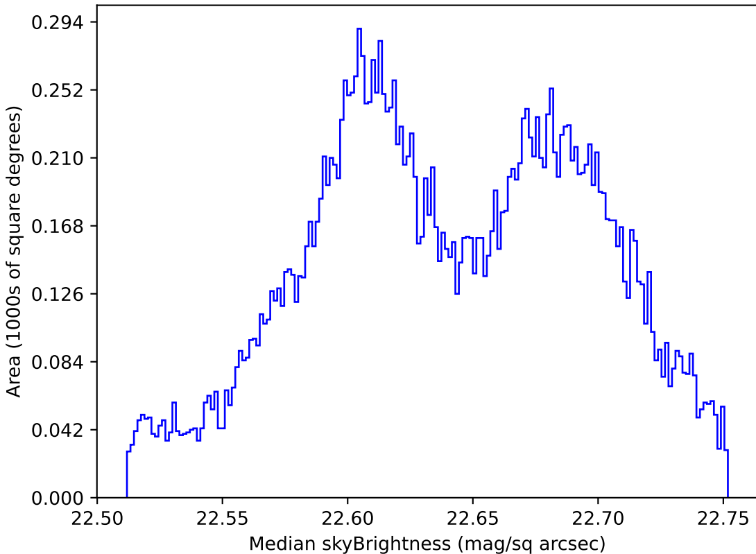
too_5_4v3.4_10yrs All sky u band: Median skyBrightness
