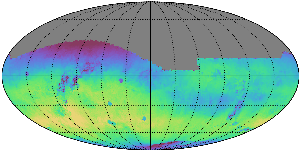
too_5_4v3.4_10yrs All sky r band: Median skyBrightness
