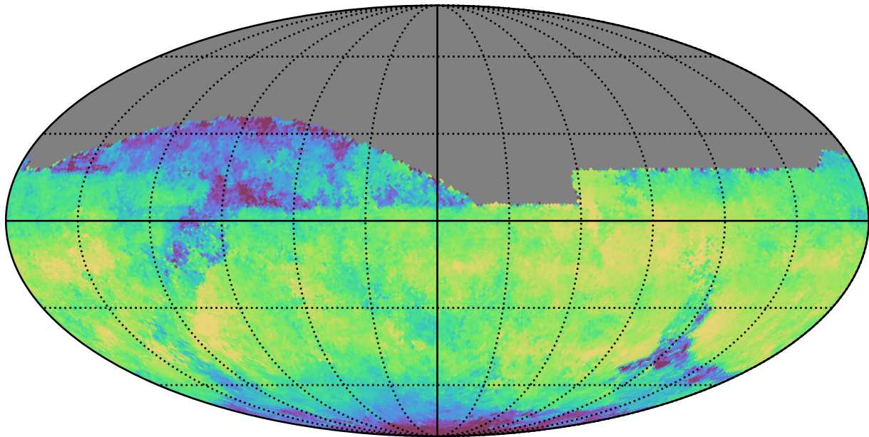
too_5_4v3.4_10yrs All sky i band: Median skyBrightness
