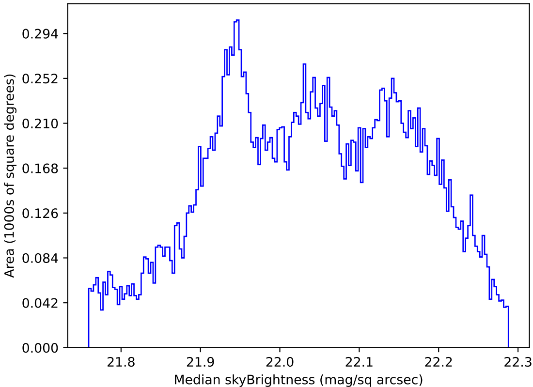
too_5_4v3.4_10yrs All sky g band: Median skyBrightness
