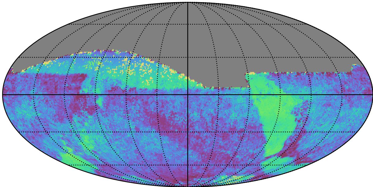
too_5_4v3.4_10yrs All sky all bands: Median skyBrightness
