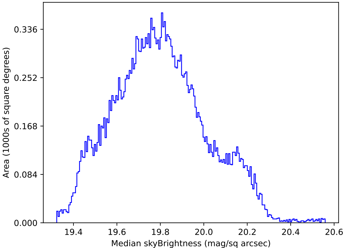
too_5_4v3.4_10yrs All sky all bands: Median skyBrightness
