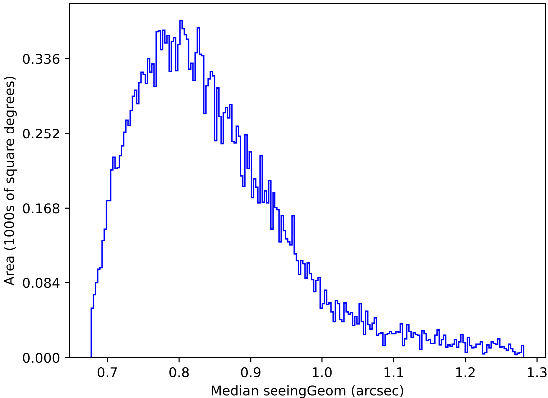
too_5_4v3.4_10yrs Yr 1 z band: Median seeingGeom
