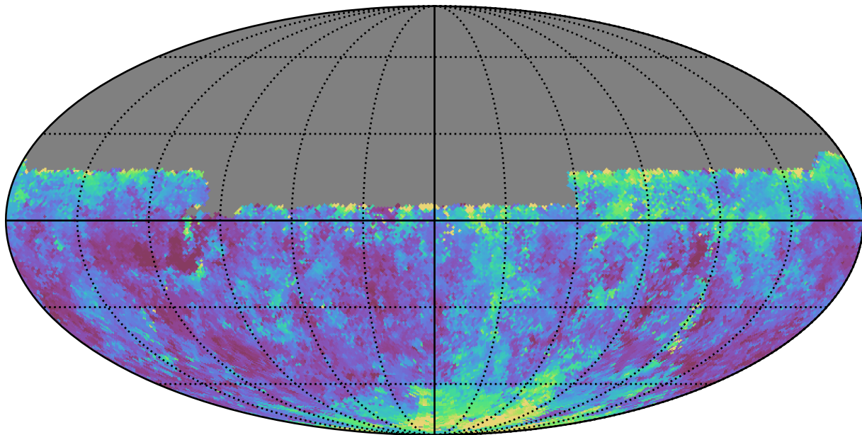
too_5_4v3.4_10yrs Yr 1 y band: Median seeingGeom
