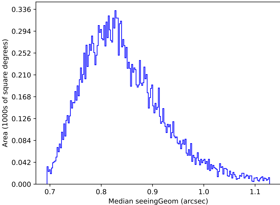
too_5_4v3.4_10yrs Yr 1 y band: Median seeingGeom
