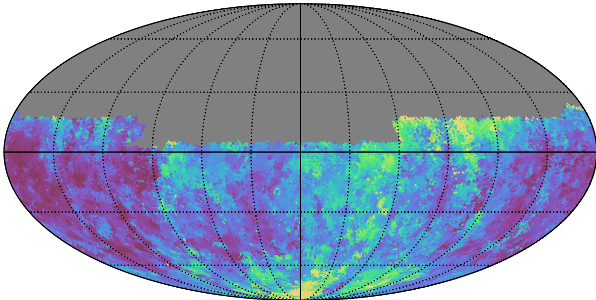
too_5_4v3.4_10yrs Yr 1 u band: Median seeingGeom
