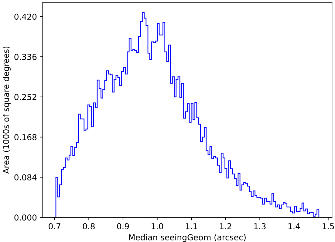
too_5_4v3.4_10yrs Yr 1 u band: Median seeingGeom
