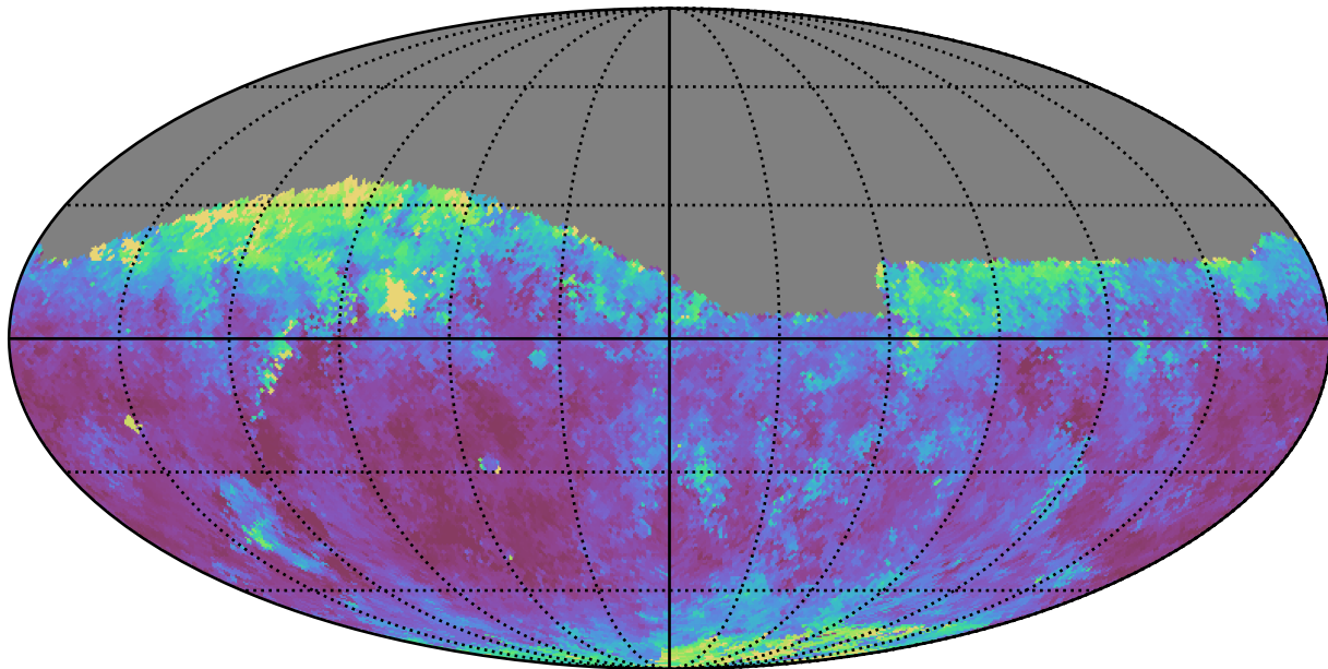
too_5_4v3.4_10yrs Yr 1 i band: Median seeingGeom
