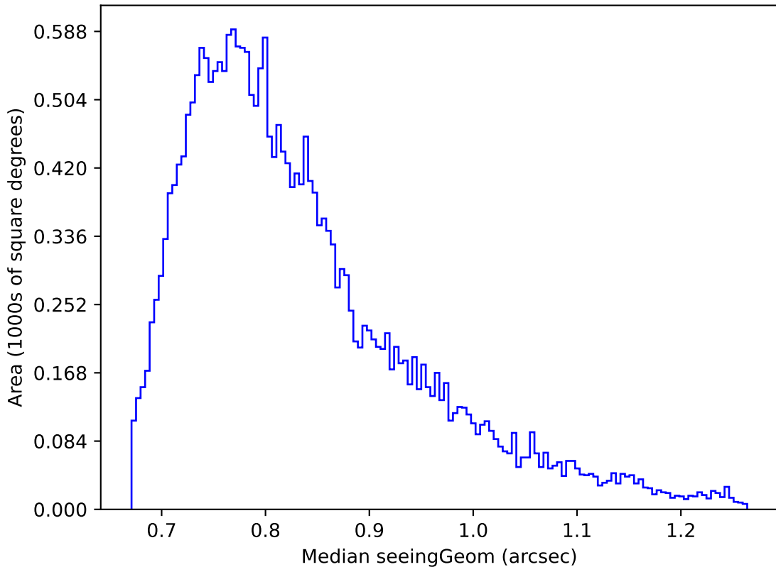
too_5_4v3.4_10yrs Yr 1 i band: Median seeingGeom
