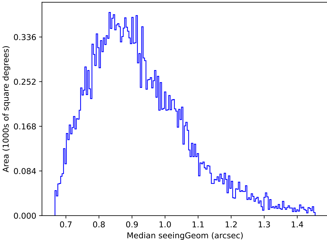
too_5_4v3.4_10yrs Yr 1 g band: Median seeingGeom
