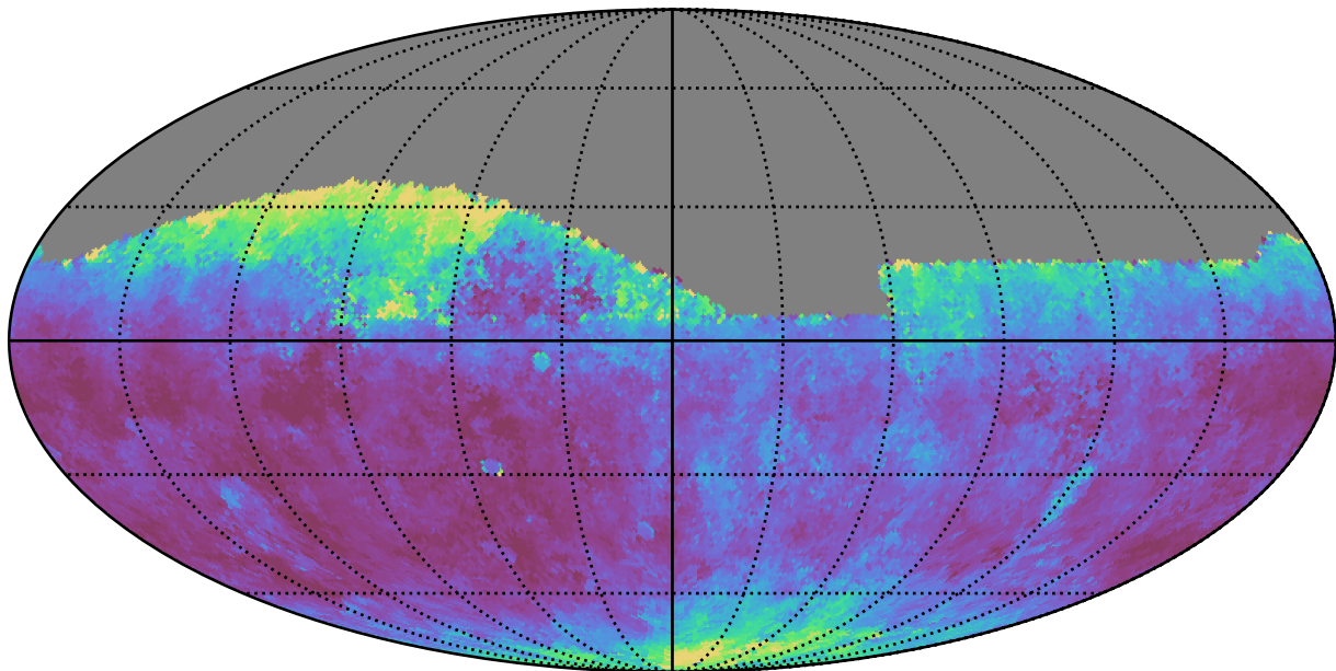
too_5_4v3.4_10yrs Yr 1 all bands: Median seeingGeom
