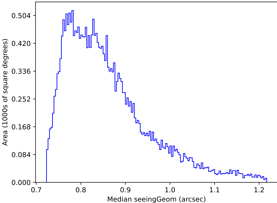
too_5_4v3.4_10yrs Yr 1 all bands: Median seeingGeom
