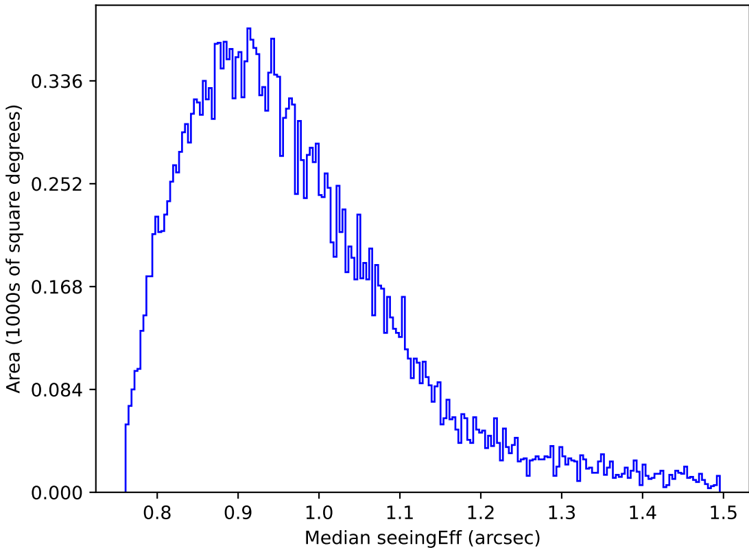
too_5_4v3.4_10yrs Yr 1 z band: Median seeingEff
